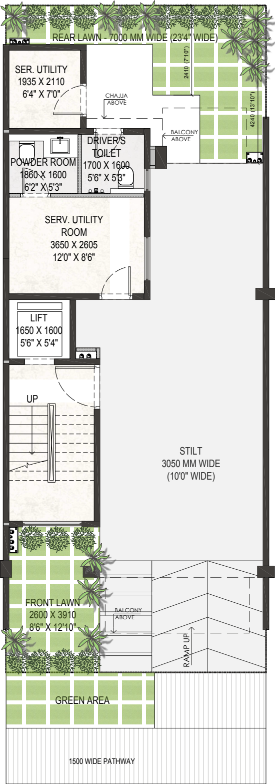
STILT FLOOR PLAN
